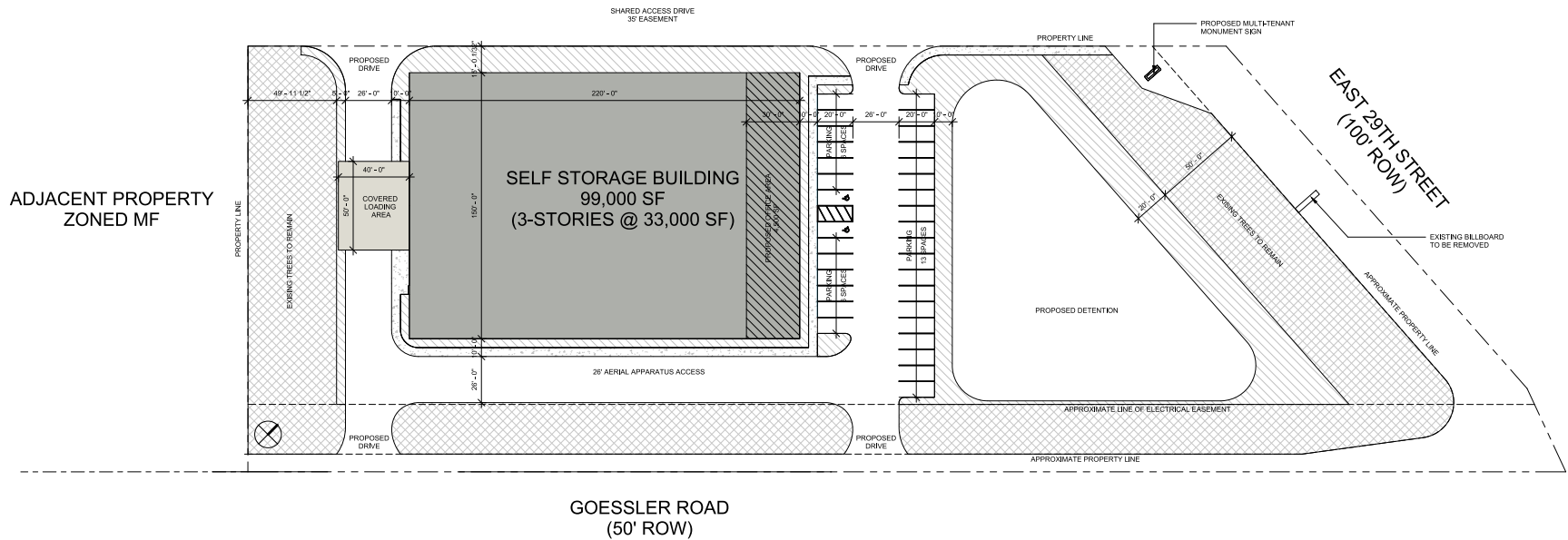
SCHEMATIC SITE PLAN 4 1" = 30'-0"
